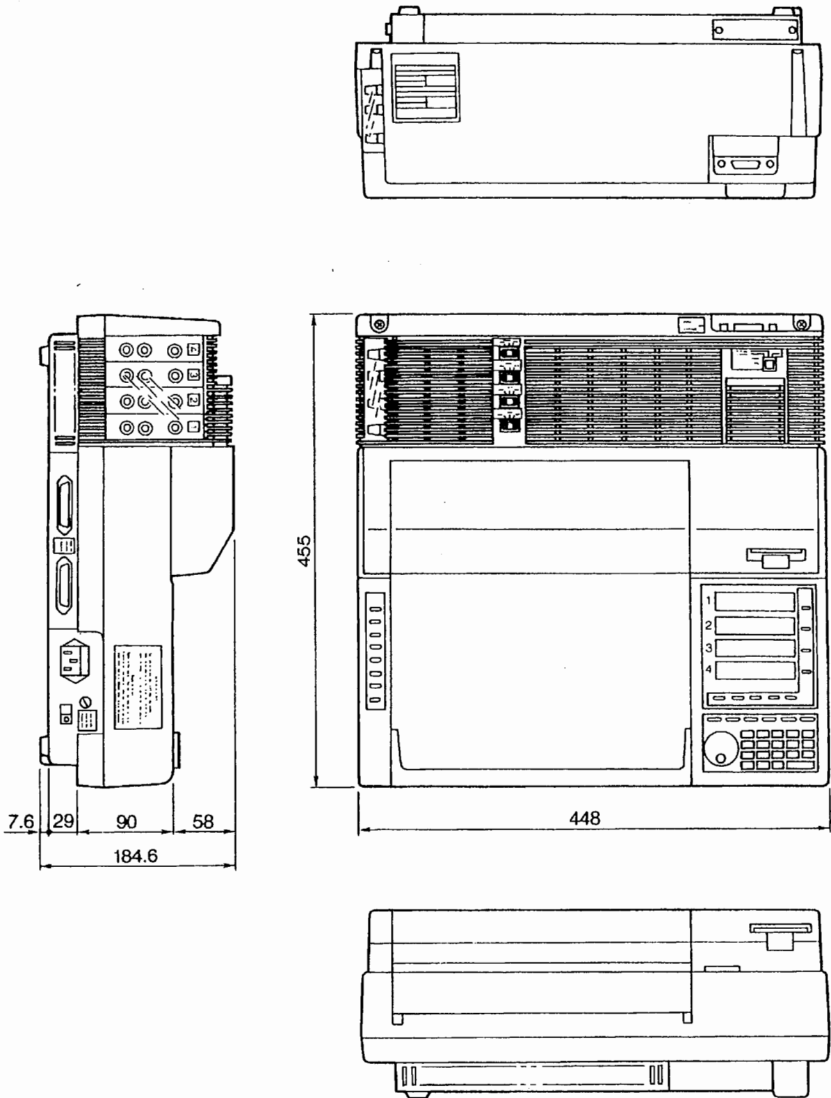
Figure 4.1 Dimensions
