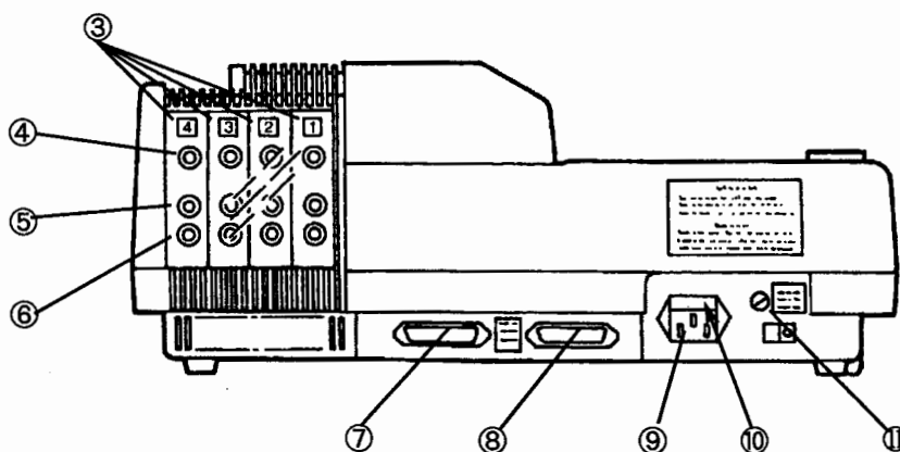
Figure 3.2 Rear Panel (4-channel model)
